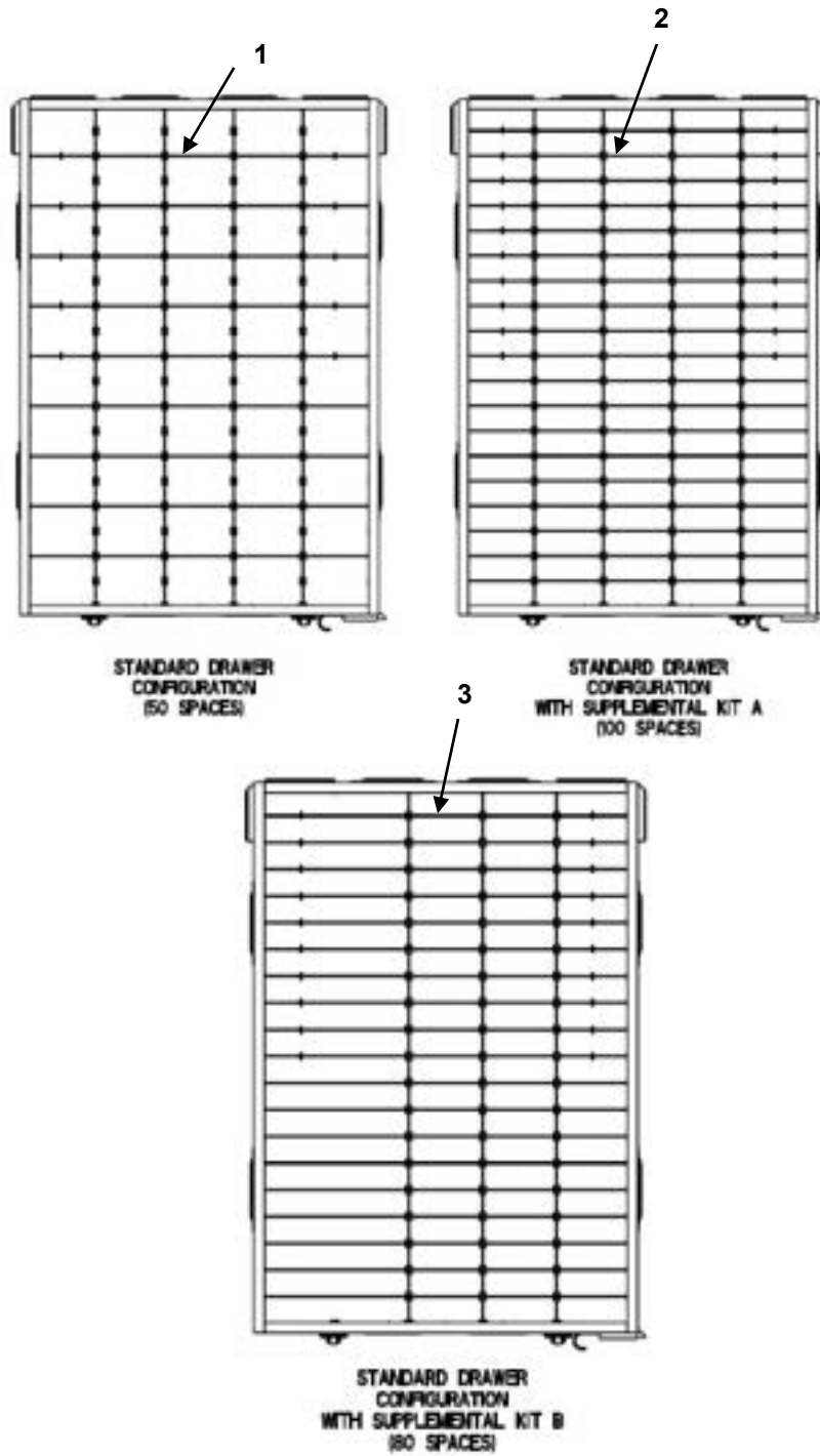
FIGURE 09 FOUR INCH DRAWER DIVIDER KITS
