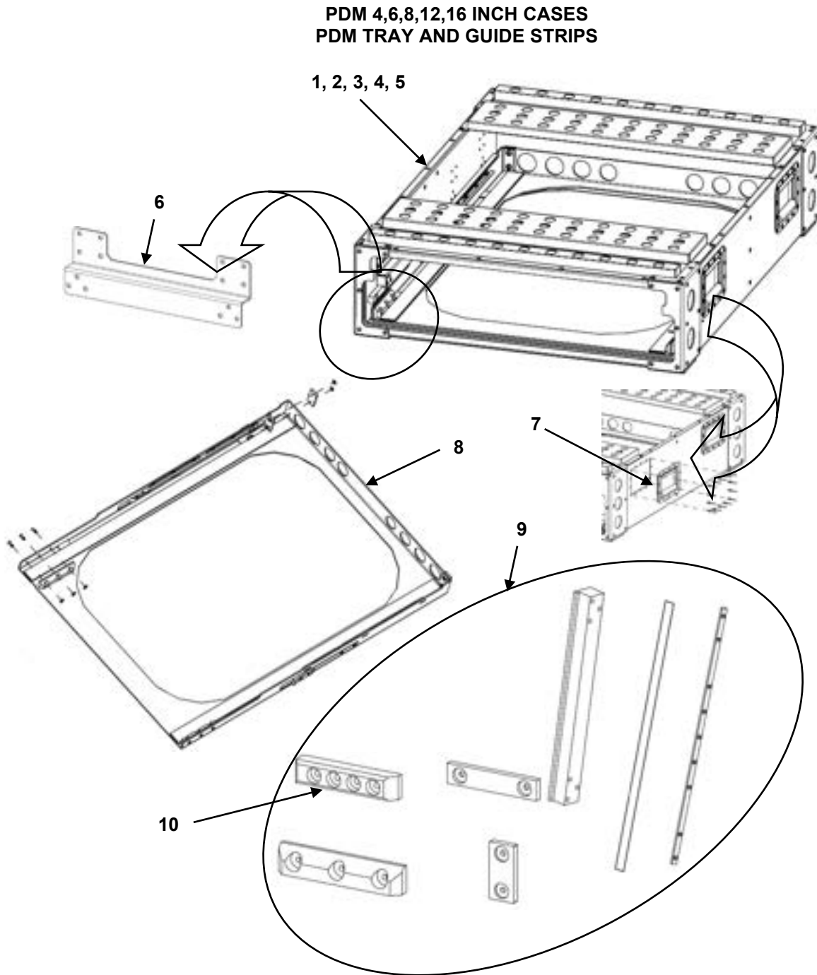
FIGURE 14 PDM 4,6,8,12,16 INCH CASES PDM TRAY AND GUIDE STRIPS
