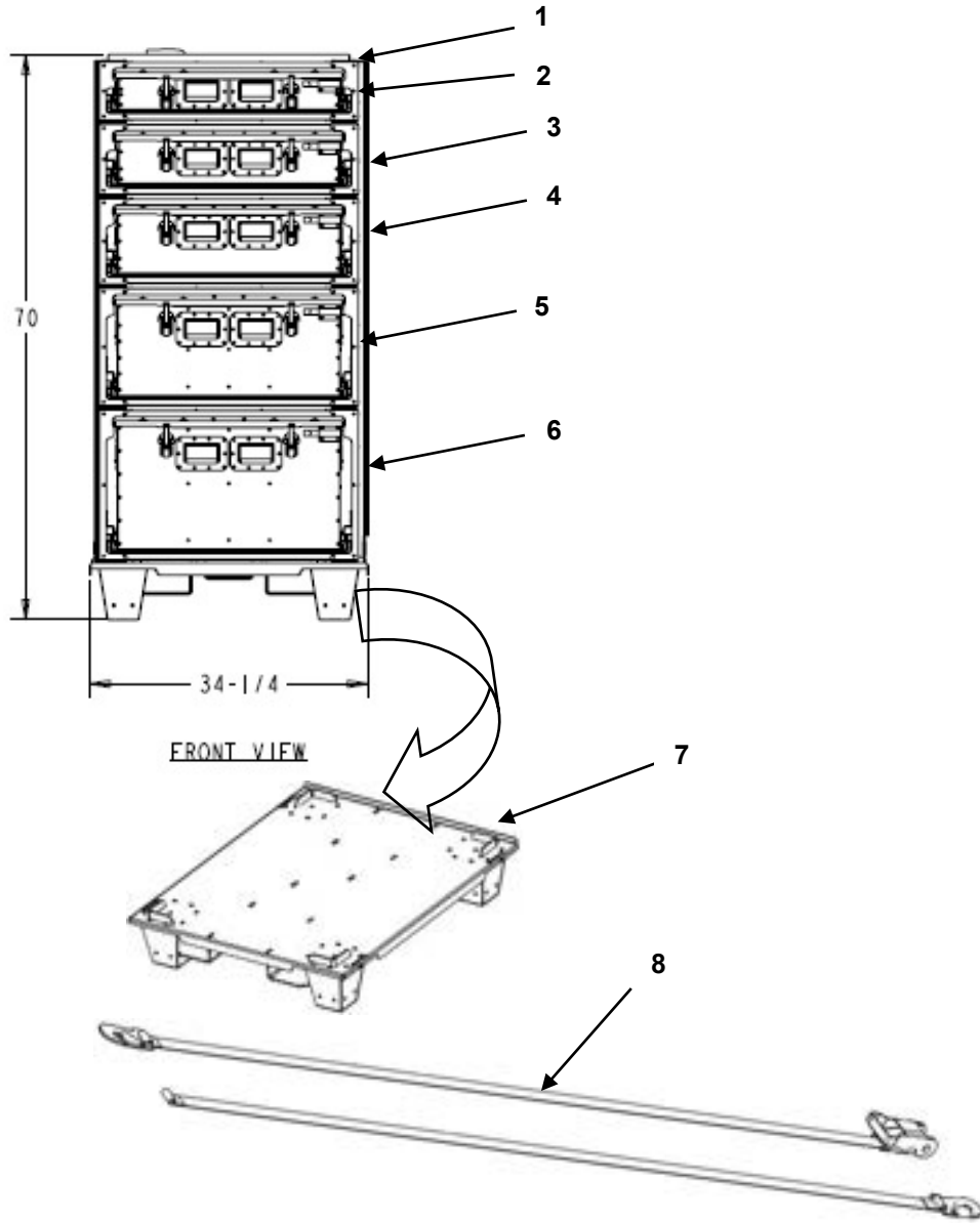
FIGURE 04 PDM CONFIGURATION # 03
