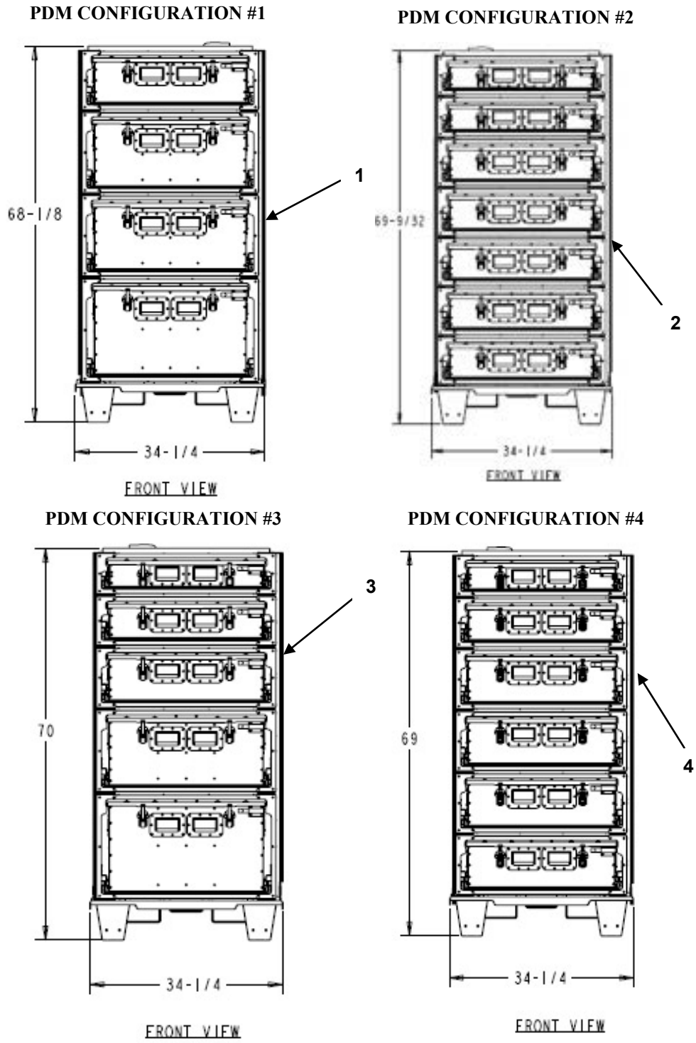
FIGURE 01 PDM CONFIGURATIONS # 01 THRU # 04
