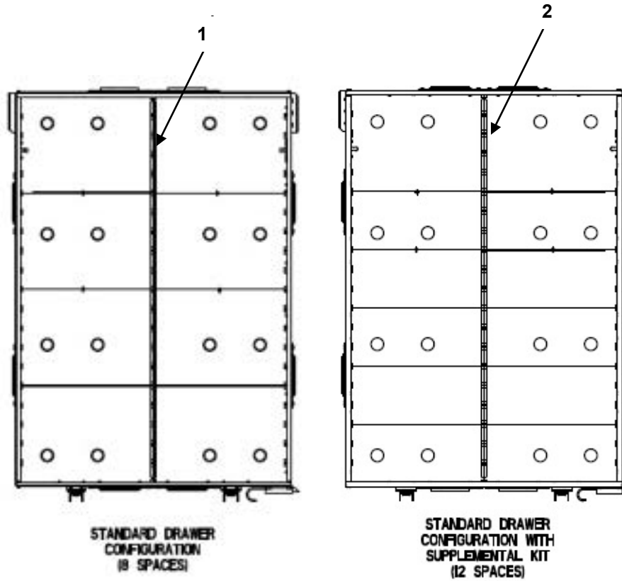
FIGURE 13 SIXTEEN INCH DRAWER DIVIDER KITS
