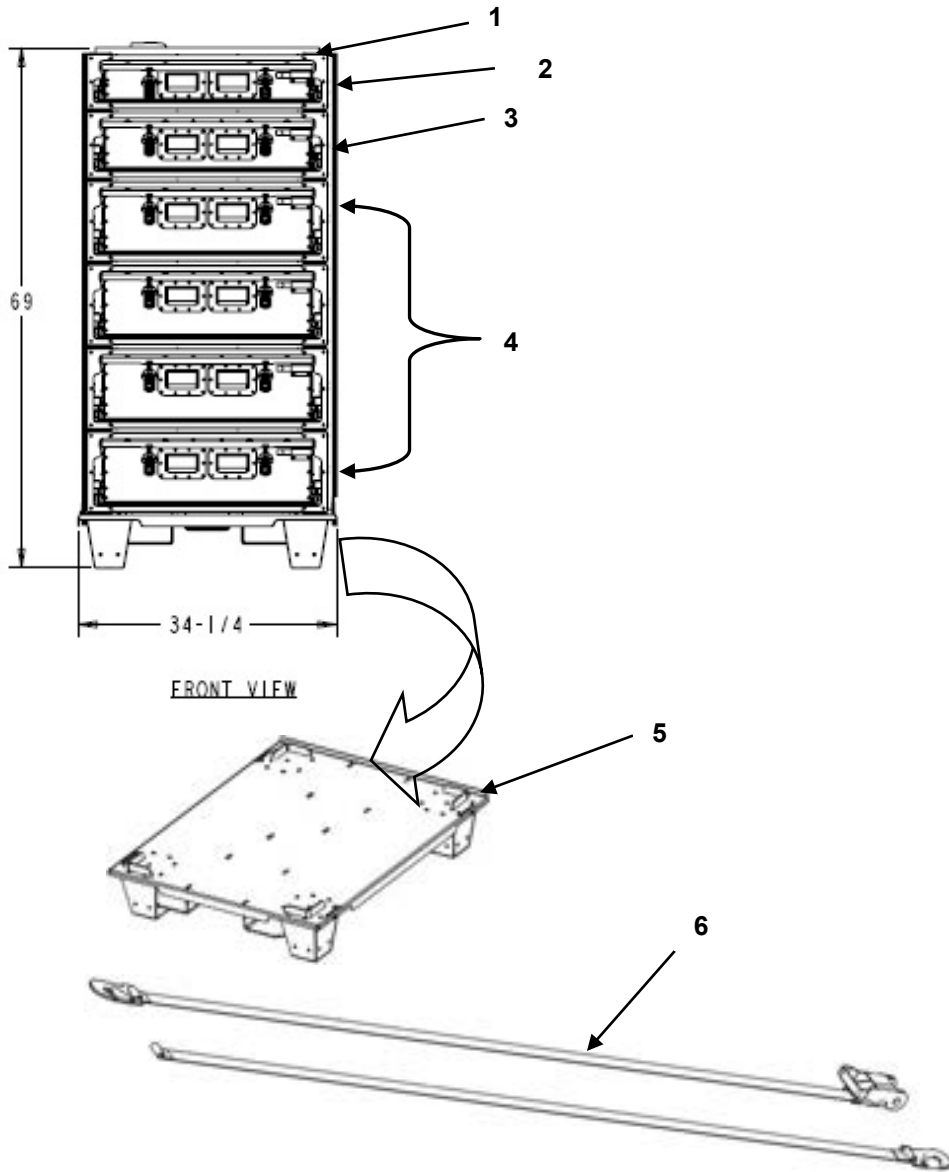
FIGURE 05 PDM CONFIGURATION # 04
