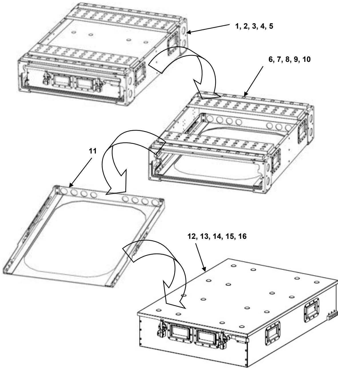
FIGURE 06 MODULE ASSEMBLIES 4", 6", 8" 12", 16" SIZES
