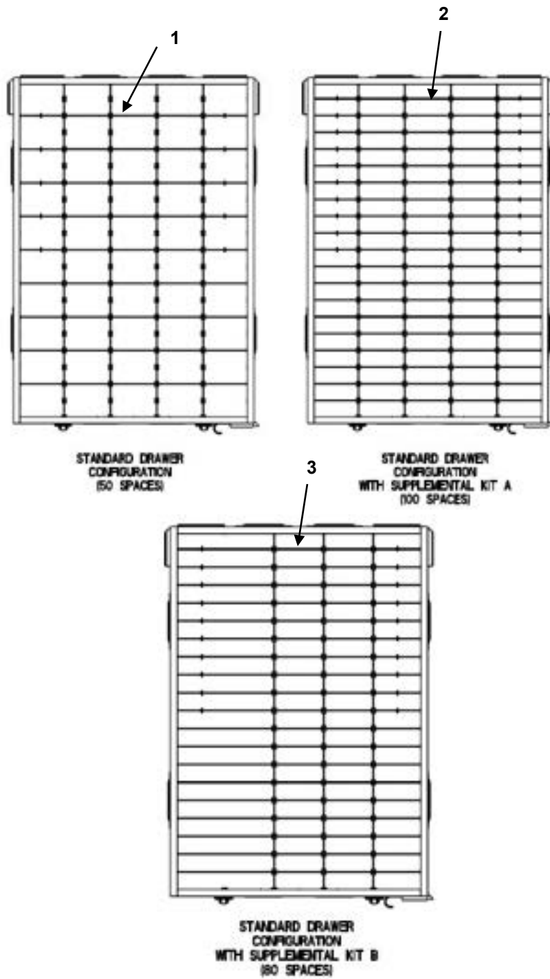
FIGURE 10 SIX INCH DRAWER DIVIDER KITS
