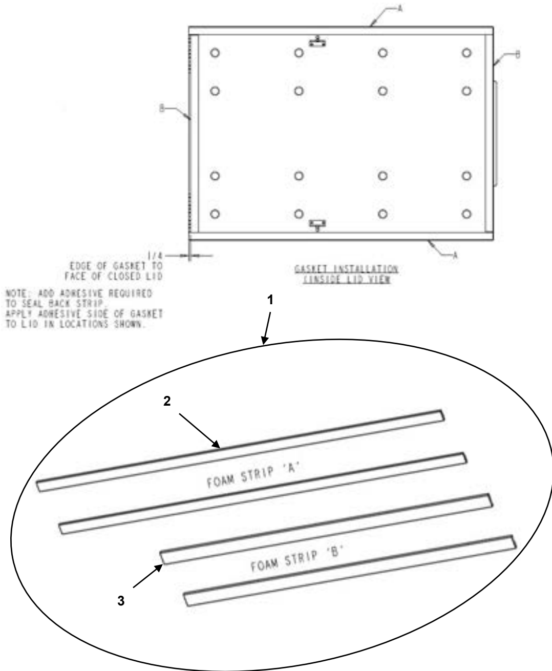
FIGURE 08 DRAWER LID SEALS KIT
