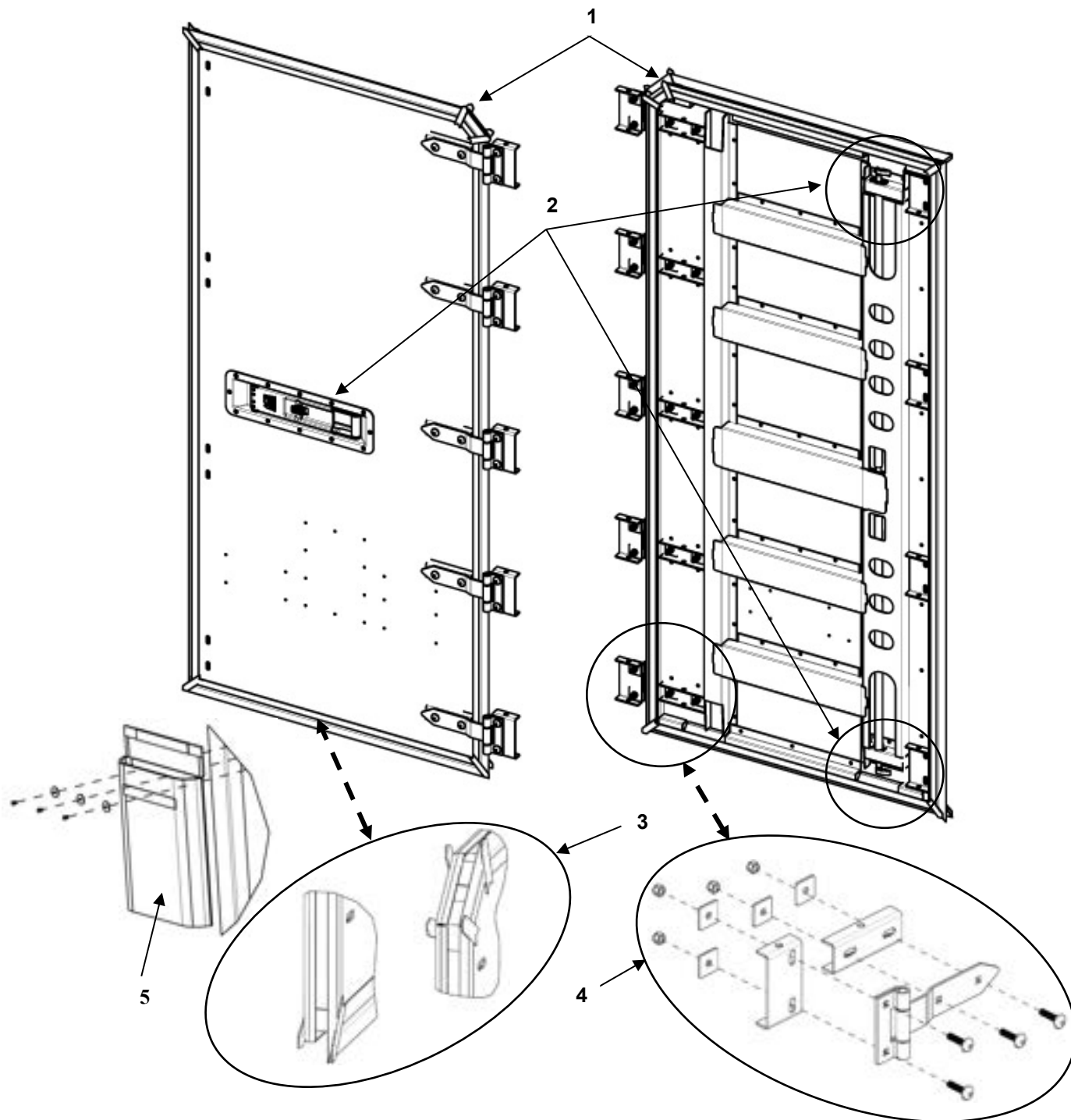
FIGURE 09 DOOR ASSEMBLY #7 BOH-CARGO-12-3 CURB SIDE
