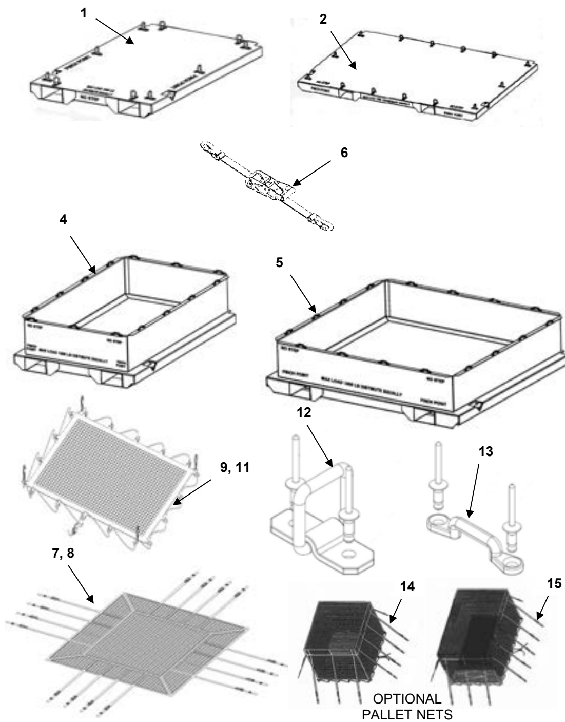
FIGURE 48 PALLETS 12 FT COMPARTMENT
