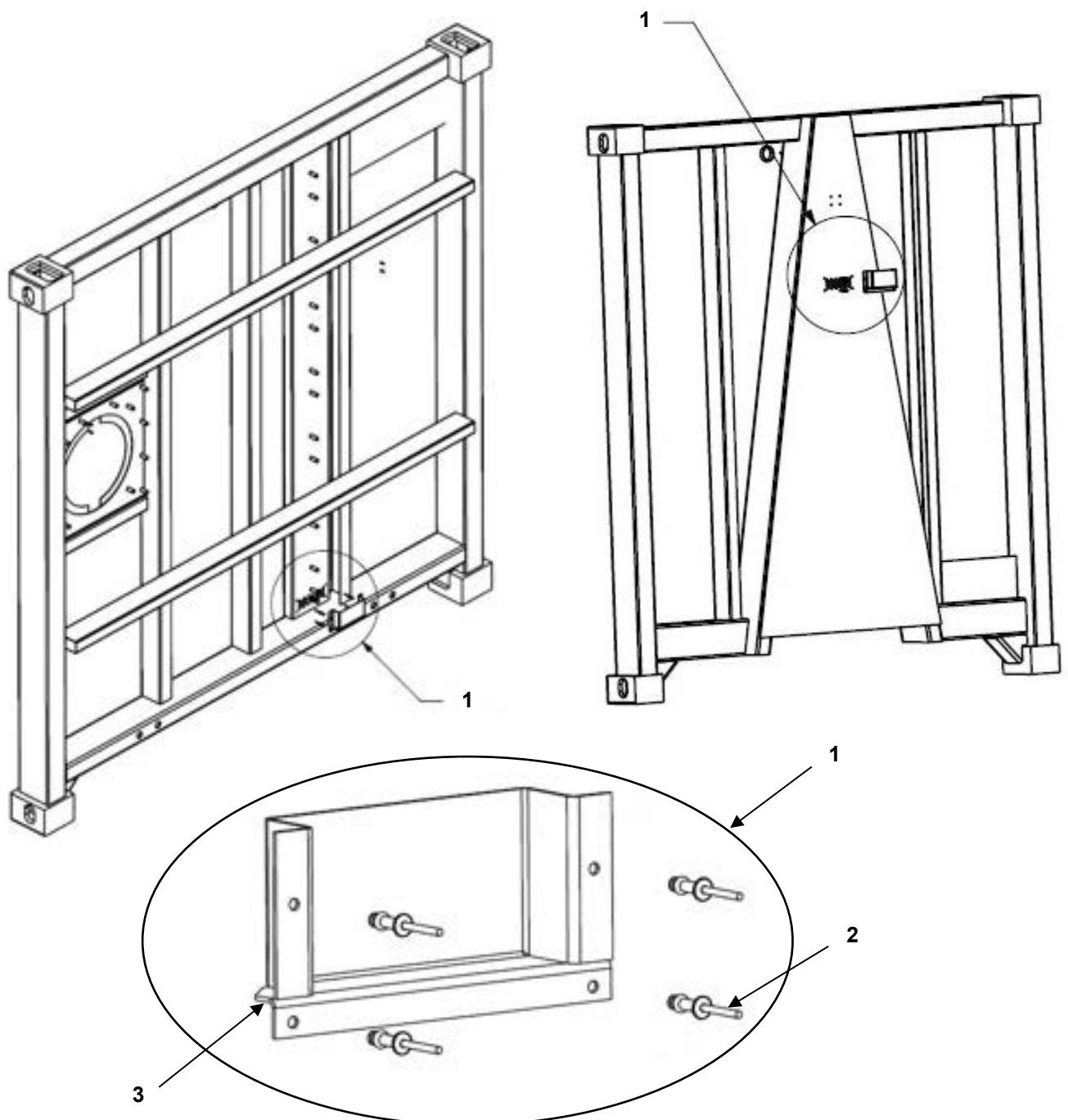
FIGURE 54 WALL VENT KIT
