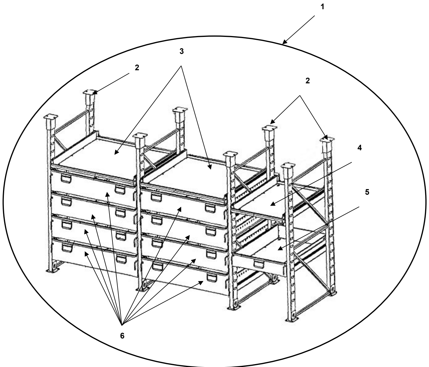
FIGURE 12 PARTS STORAGE AIDS
