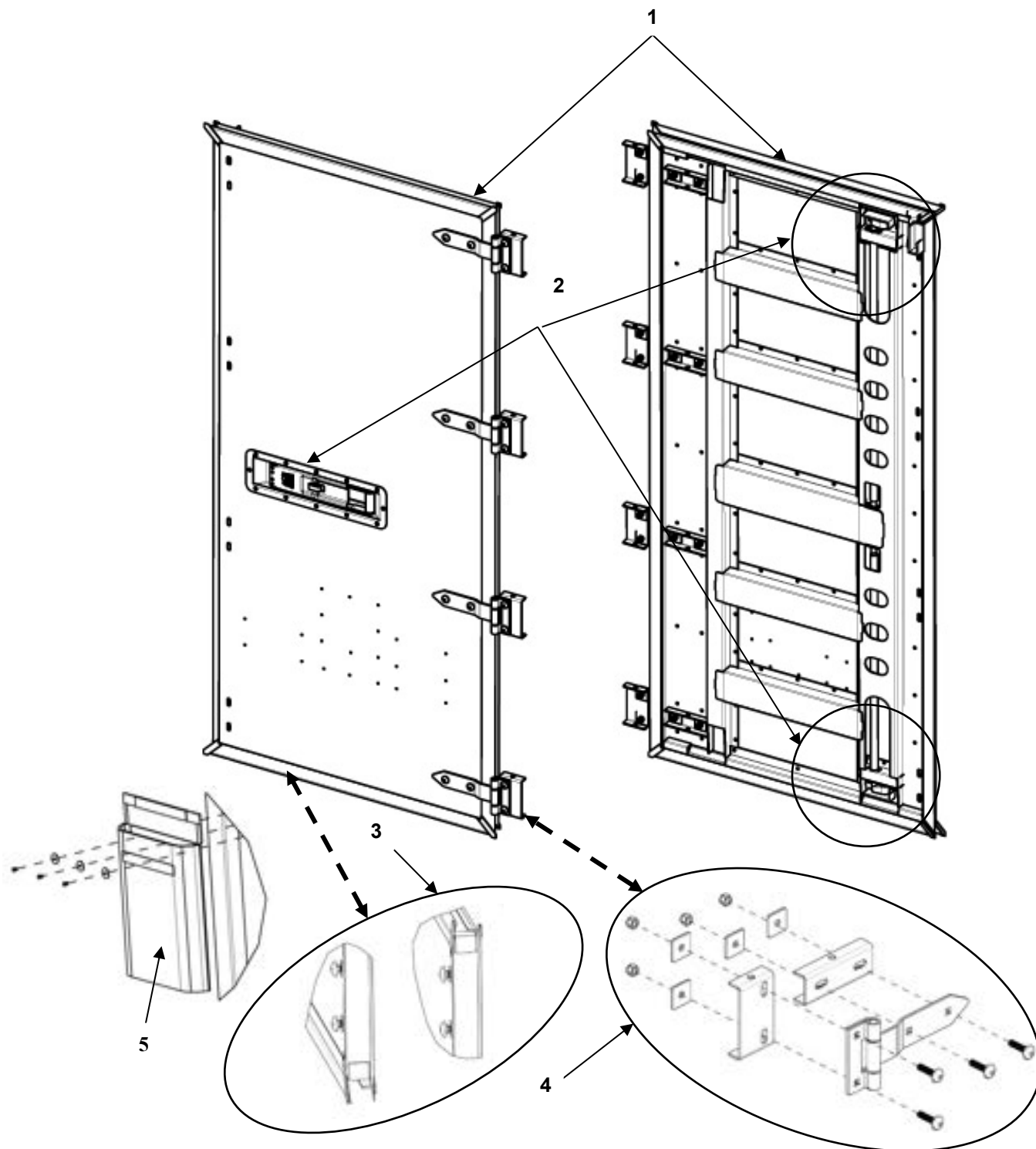
FIGURE 40 DOOR ASSEMBLY # 7
