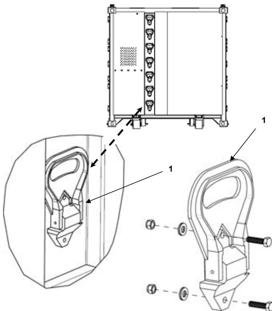
FIGURE 42 FOLDING STEPS
