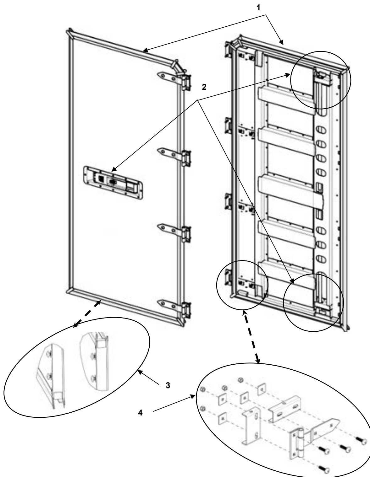
FIGURE 20 DOOR ASSEMBLY # 6
