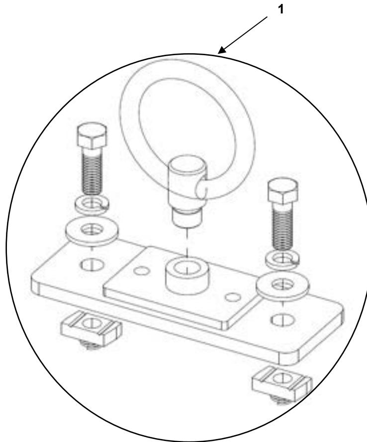
FIGURE 29 TIE DOWN RING ASSEMBLY
