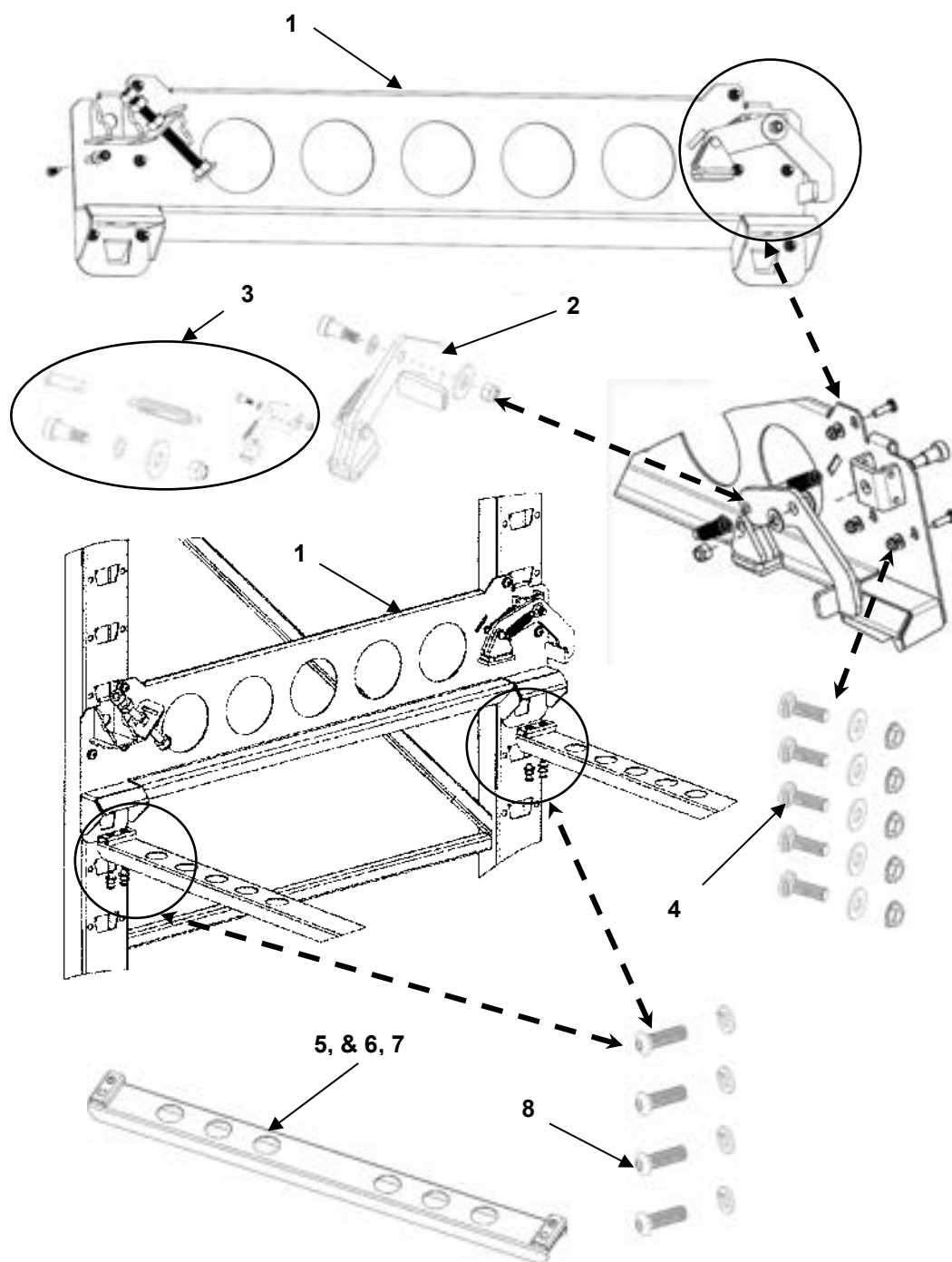
FIGURE 49 PALLET LEDGE
