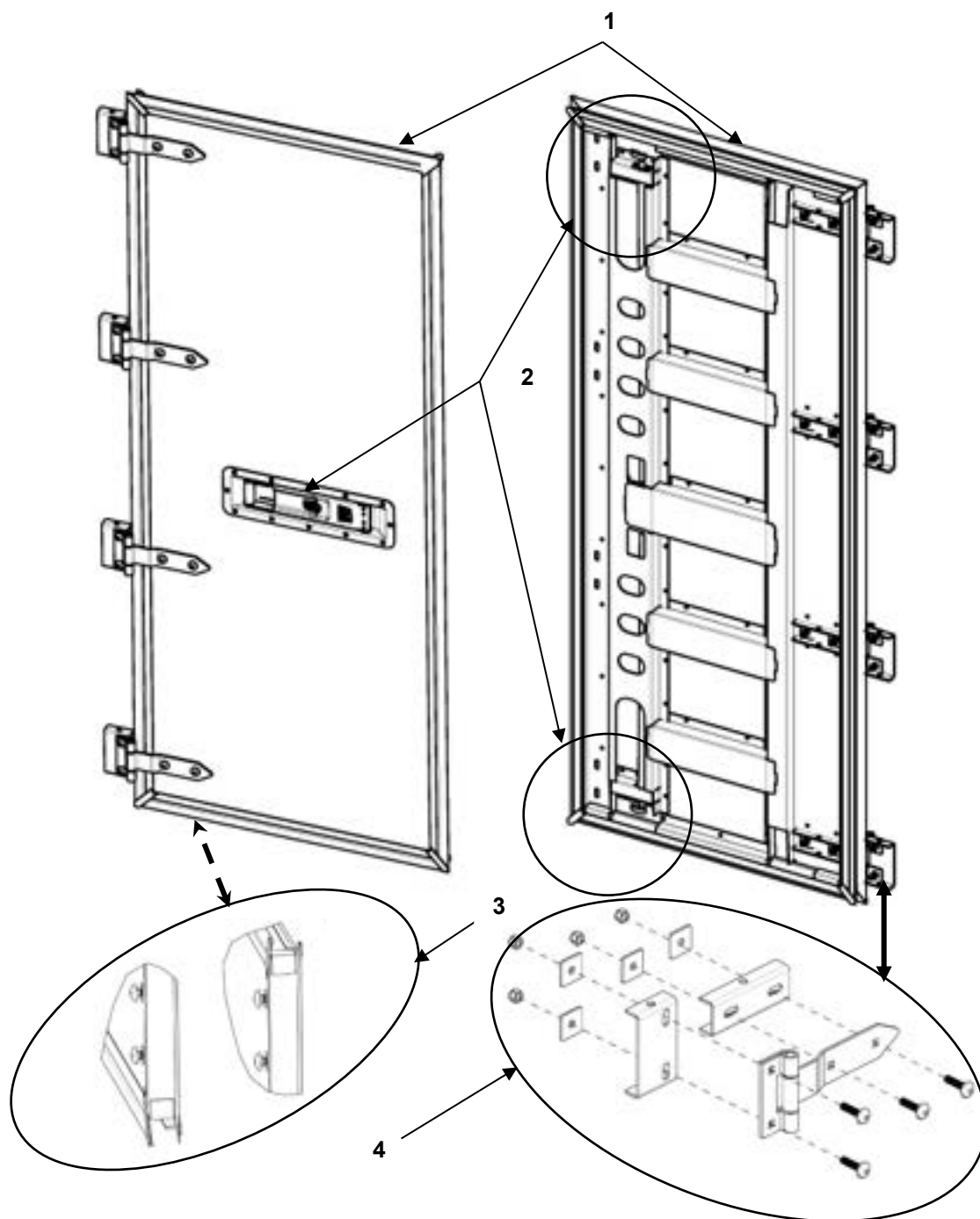
FIGURE 35 DOOR ASSEMBLY # 2 AND #9
