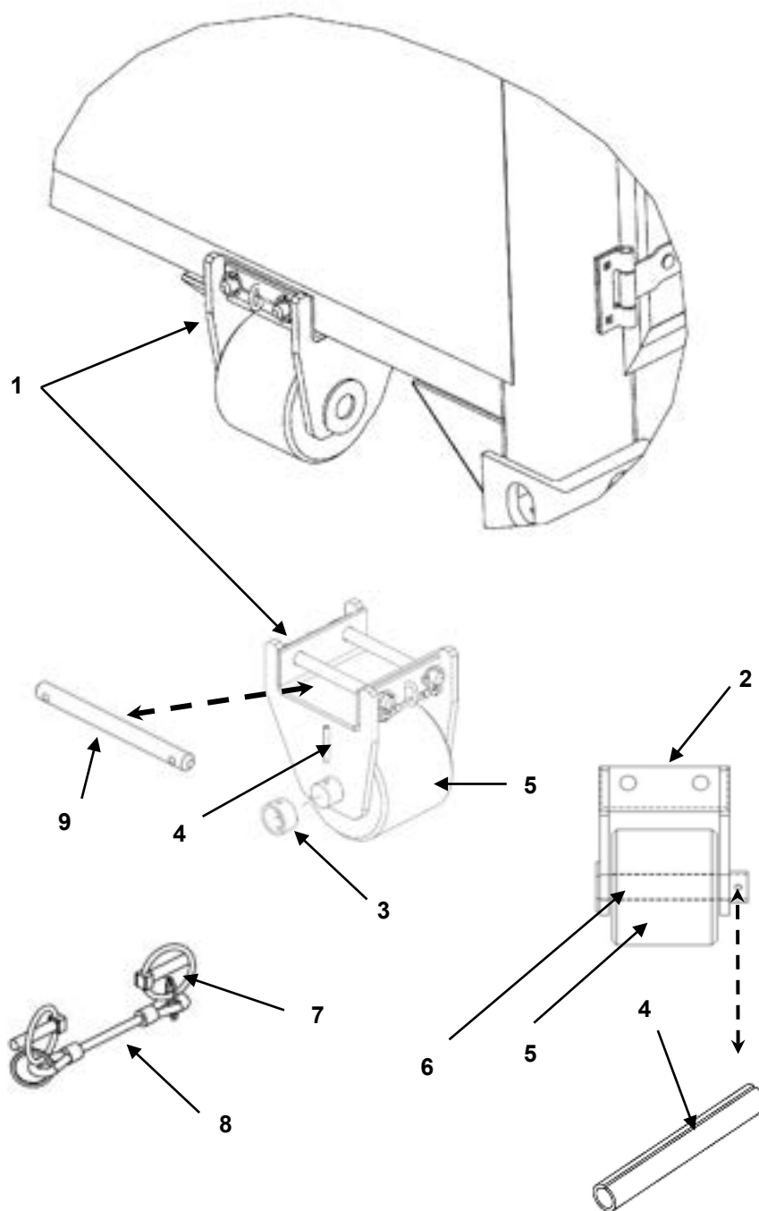
FIGURE 24 REAR ROLLER ASSEMBLY
