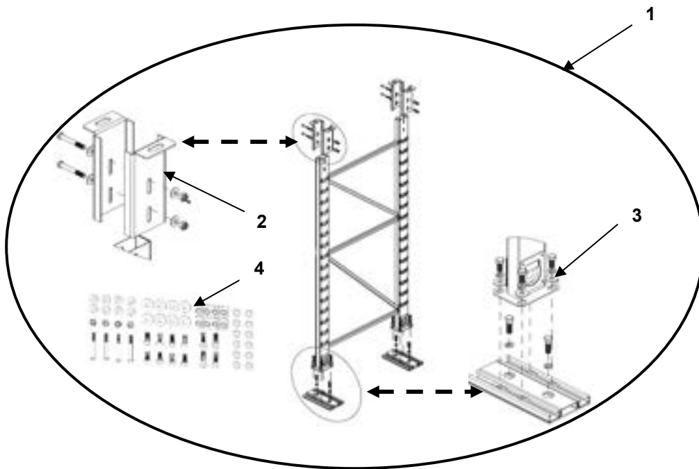
FIGURE 11 VERTICAL RACK FRAME
