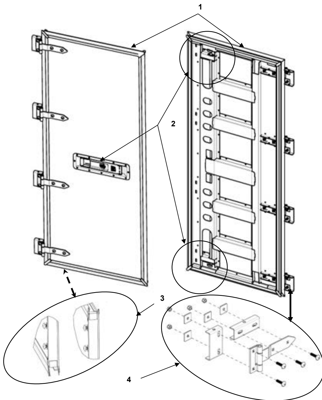
FIGURE 36 DOOR ASSEMBLIES #3 AND #8
