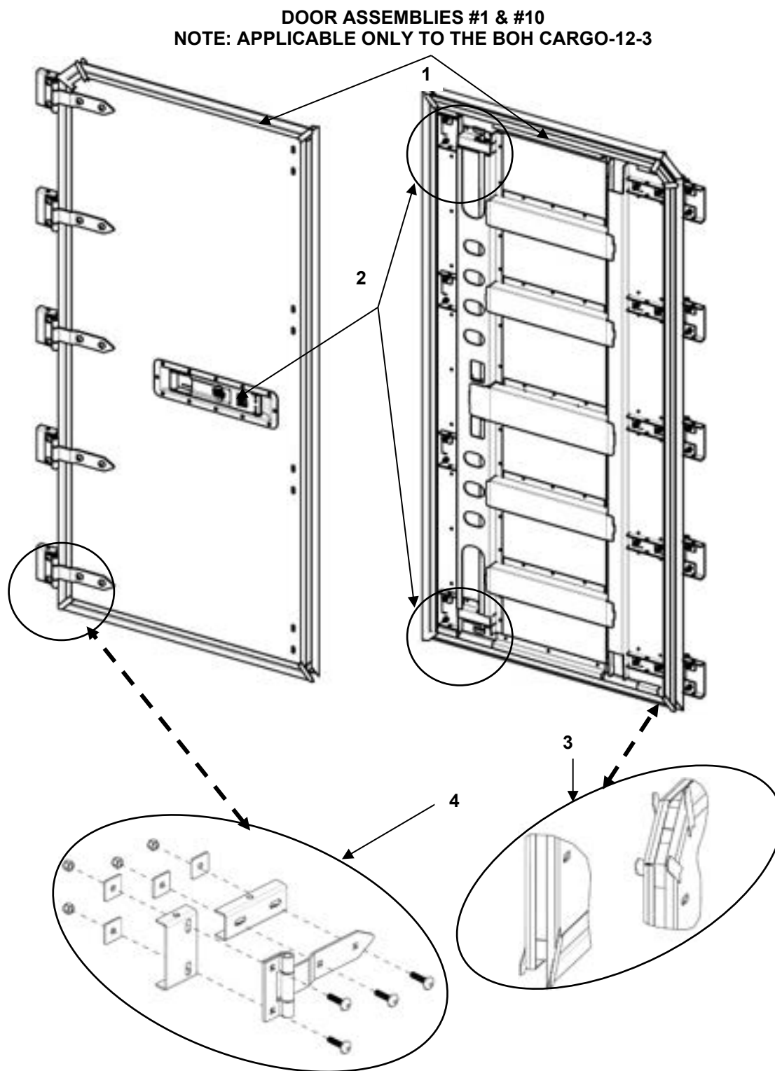
FIGURE 05 DOOR ASSEMBLIES #1 & 10 BOH-CARGO-12-3
