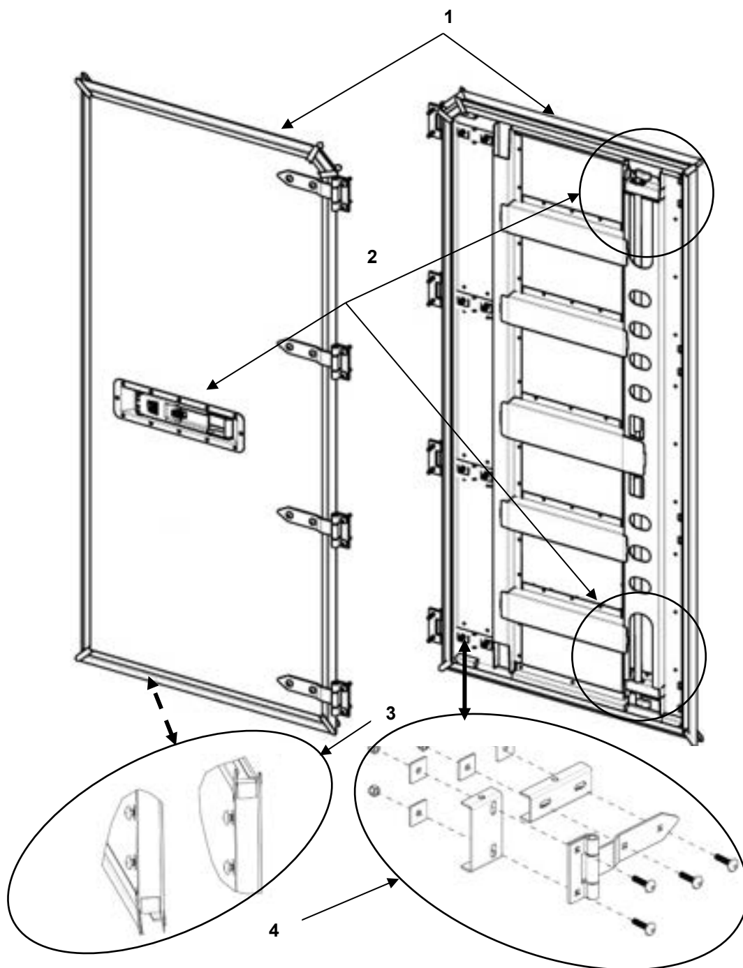
FIGURE 39 DOOR ASSEMBLIES #6 AND #11
