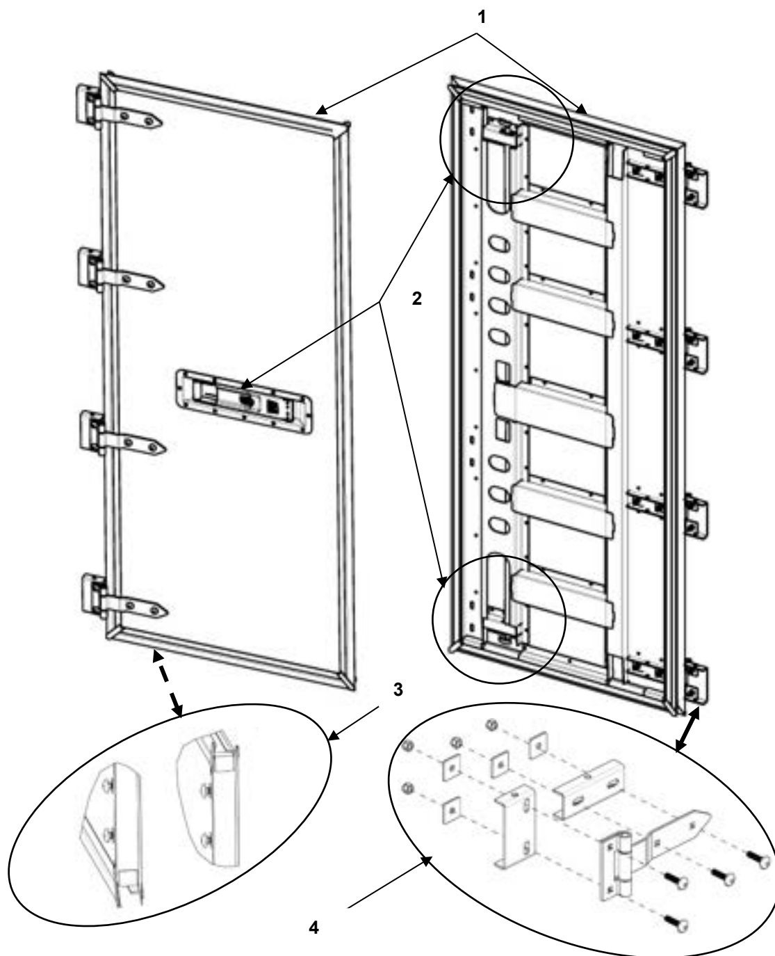
FIGURE 38 DOOR ASSEMBLIES #5 AND #12
