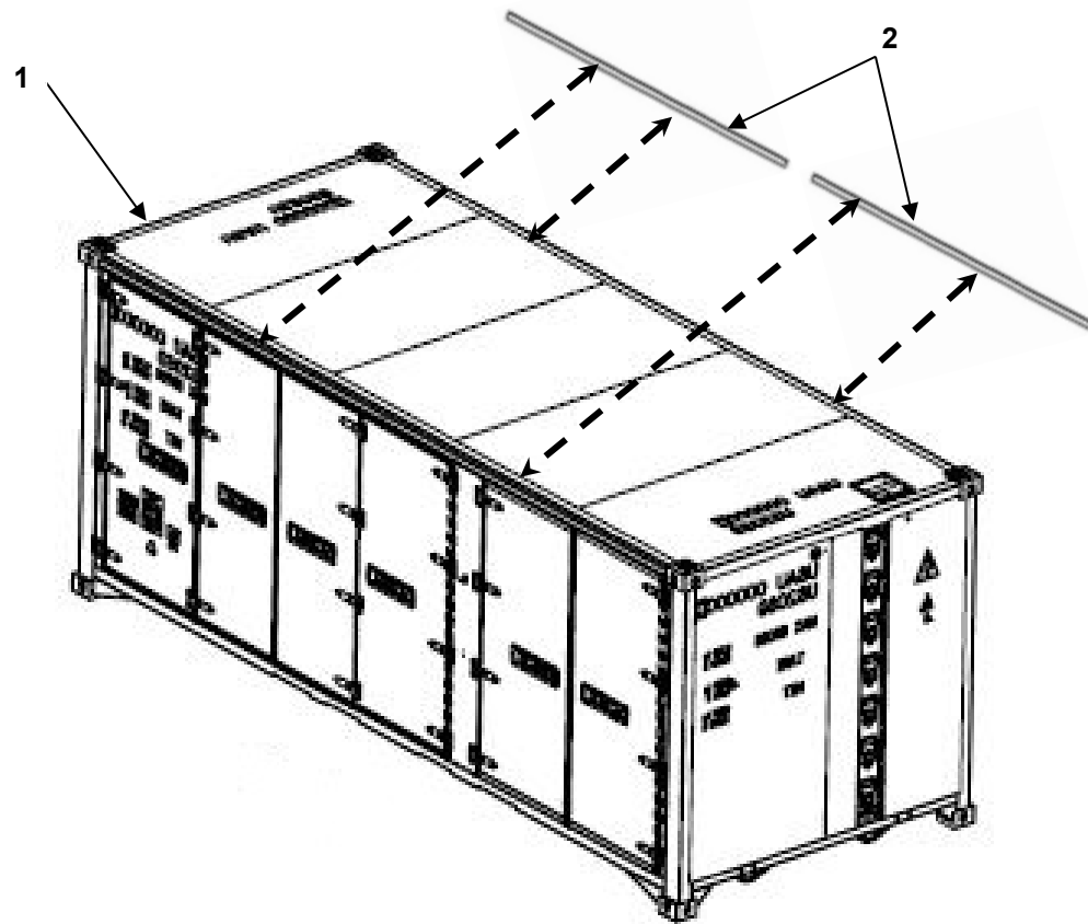
FIG 31 FPU-20-3 CONTAINER
