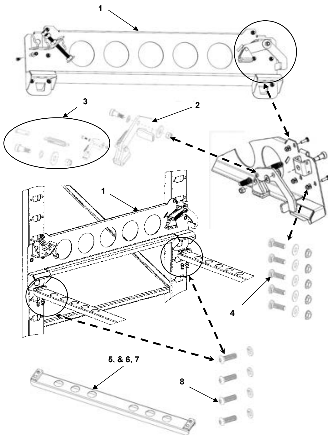
FIGURE 16 PALLET LEDGE
