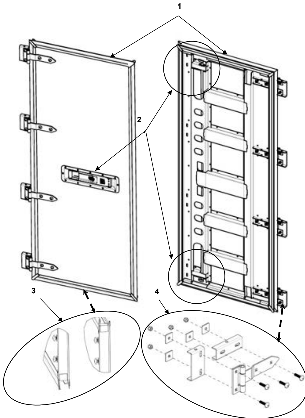
FIGURE 34 DOOR ASSEMBLIES #1 AND #10
