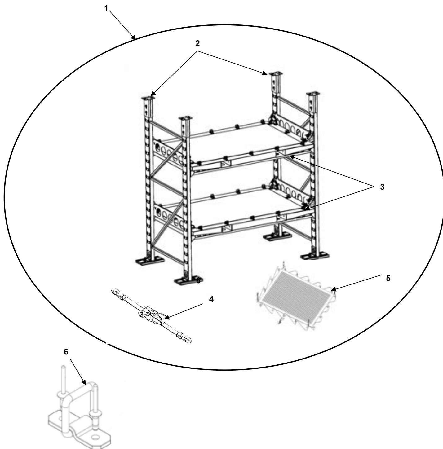
FIGURE 50 BULK STORAGE AIDS 8 FT COMPARTMENT
