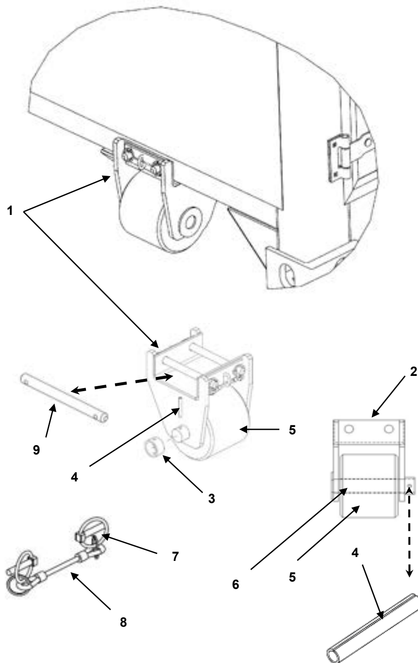
FIGURE 43 REAR ROLLER ASSEMBLY
