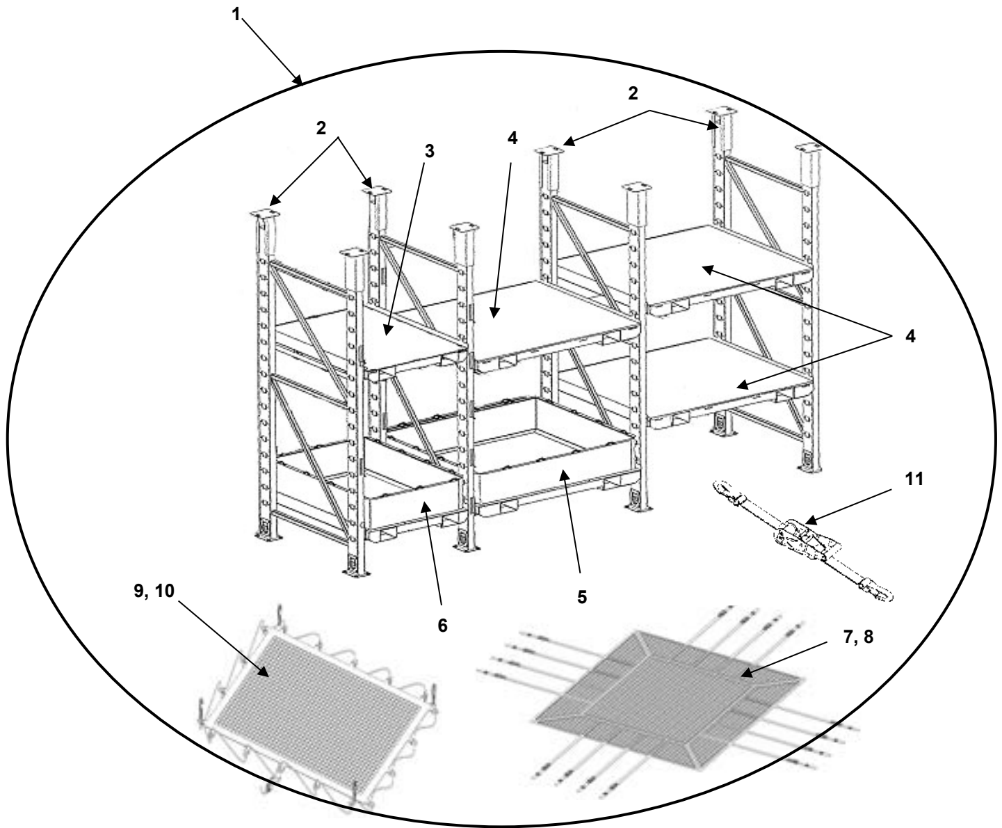
FIGURE 47 BULK STORAGE AIDS 12 FT COMPARTMENT
