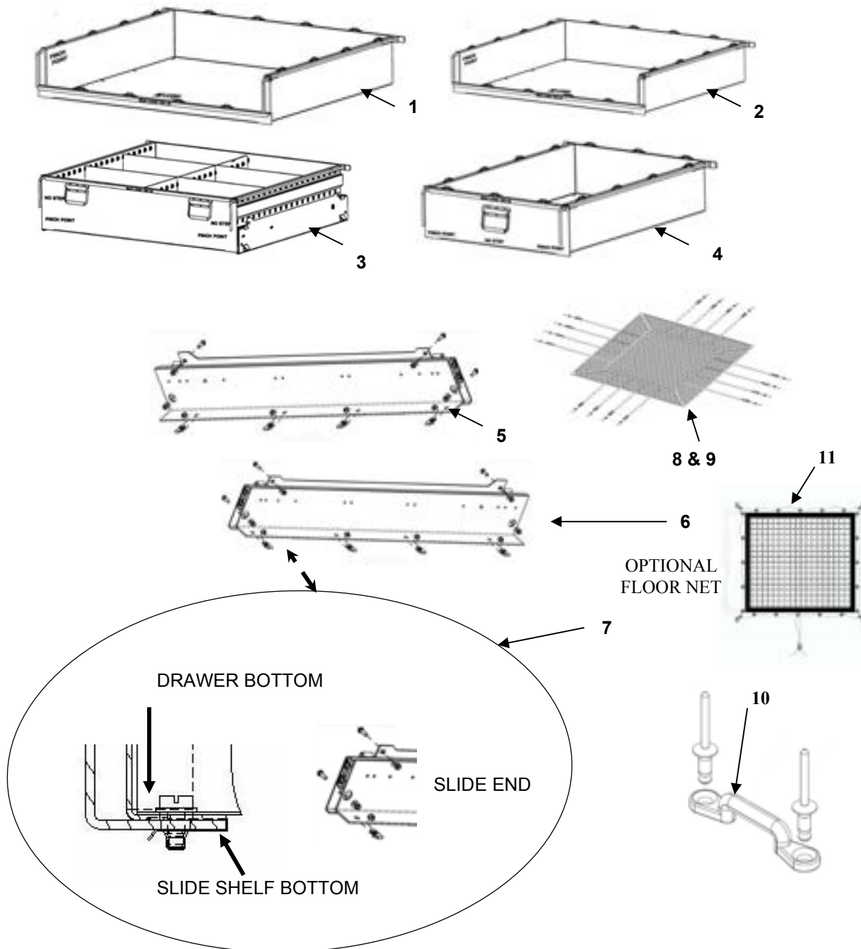
FIGURE 46 DRAWER ASSEMBLIES
