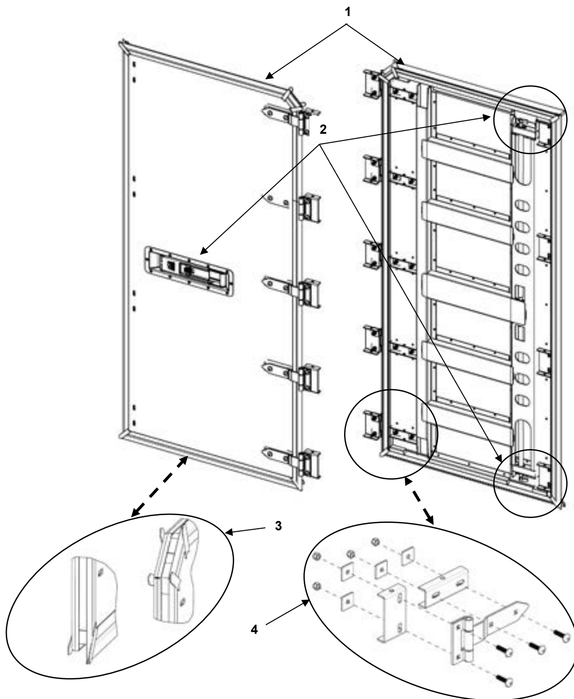
FIGURE 08 DOOR ASSEMBLY #4 BOH-CARGO-12-3 STREET SIDE
