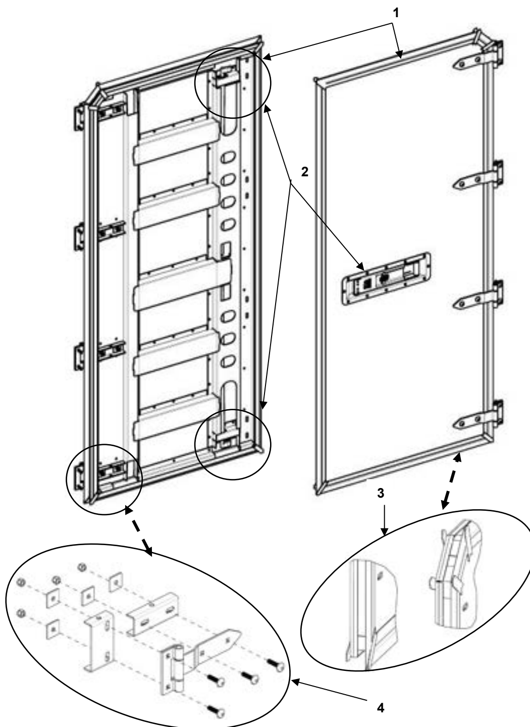
FIGURE 07 DOOR ASSEMBLIES # 3 & # 8 BOH CARGO-12-3
