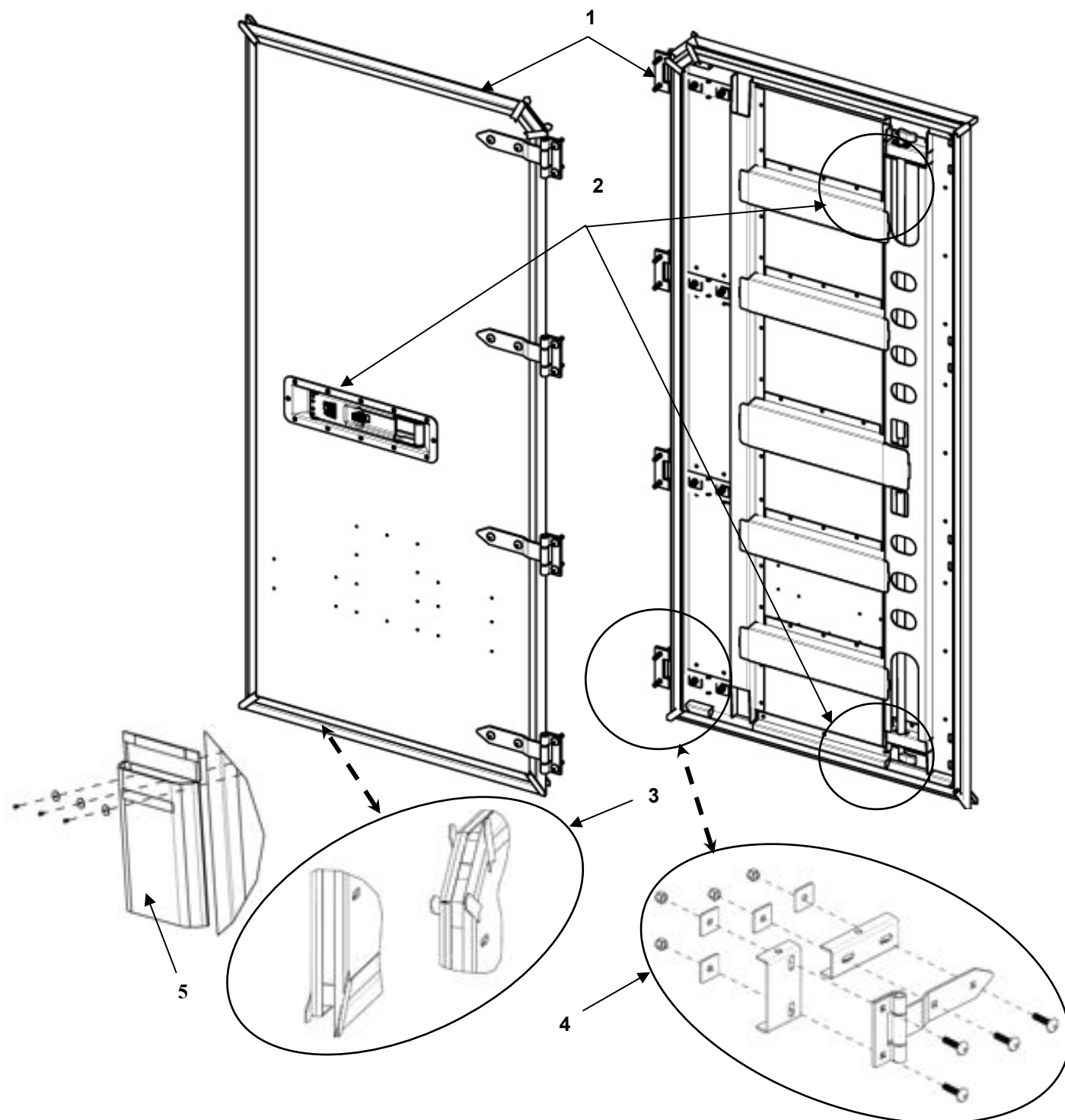
FIGURE 21 DOOR ASSEMBLY #11 FPU-8-4
