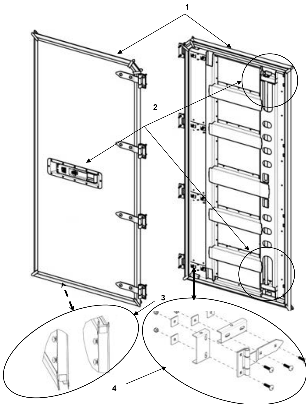
FIGURE 37 DOOR ASSEMBLY # 4
