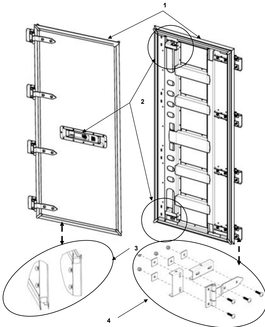
FIGURE 06 DOOR ASSEMBLIES # 2 & # 9 BOH CARGO-12-3
