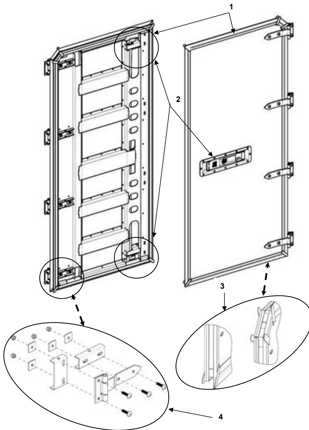
FIGURE 19 DOOR ASSEMBLIES # 5 AND #12
