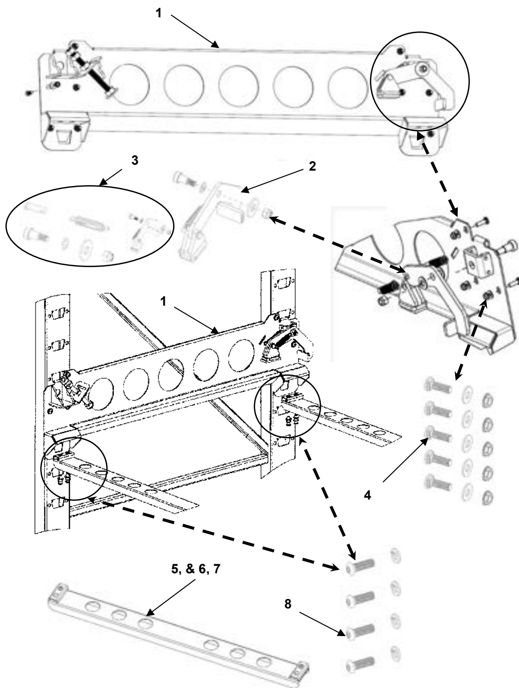
FIGURE 28 PALLET LEDGE
