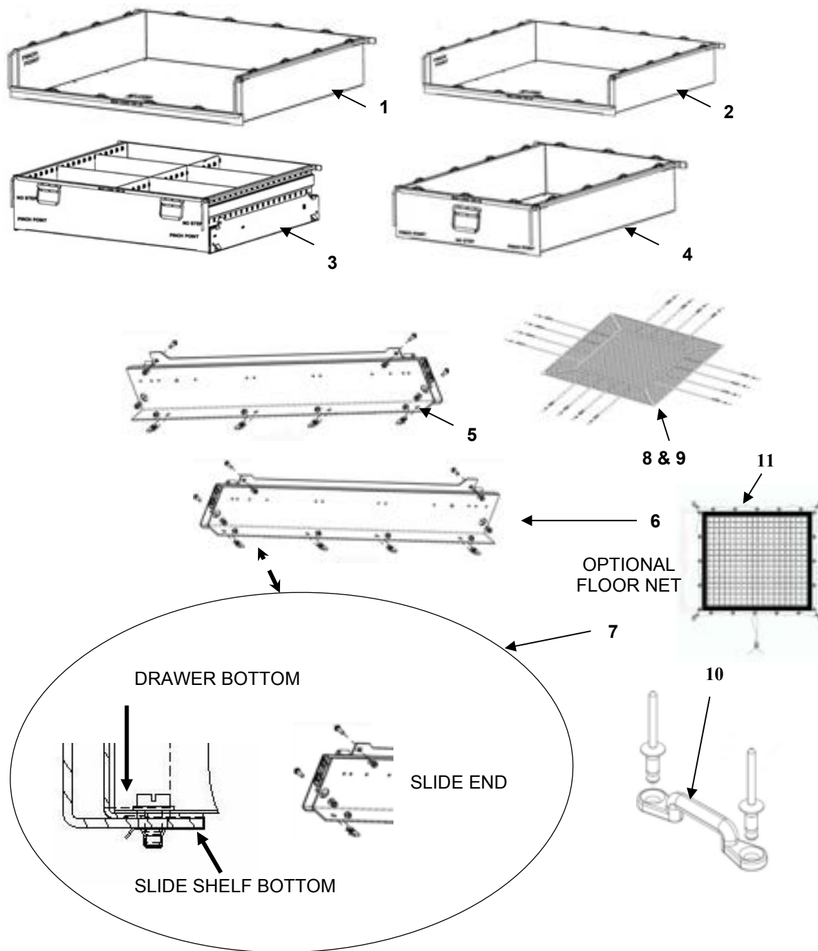
FIGURE 13 DRAWER ASSEMBLIES
