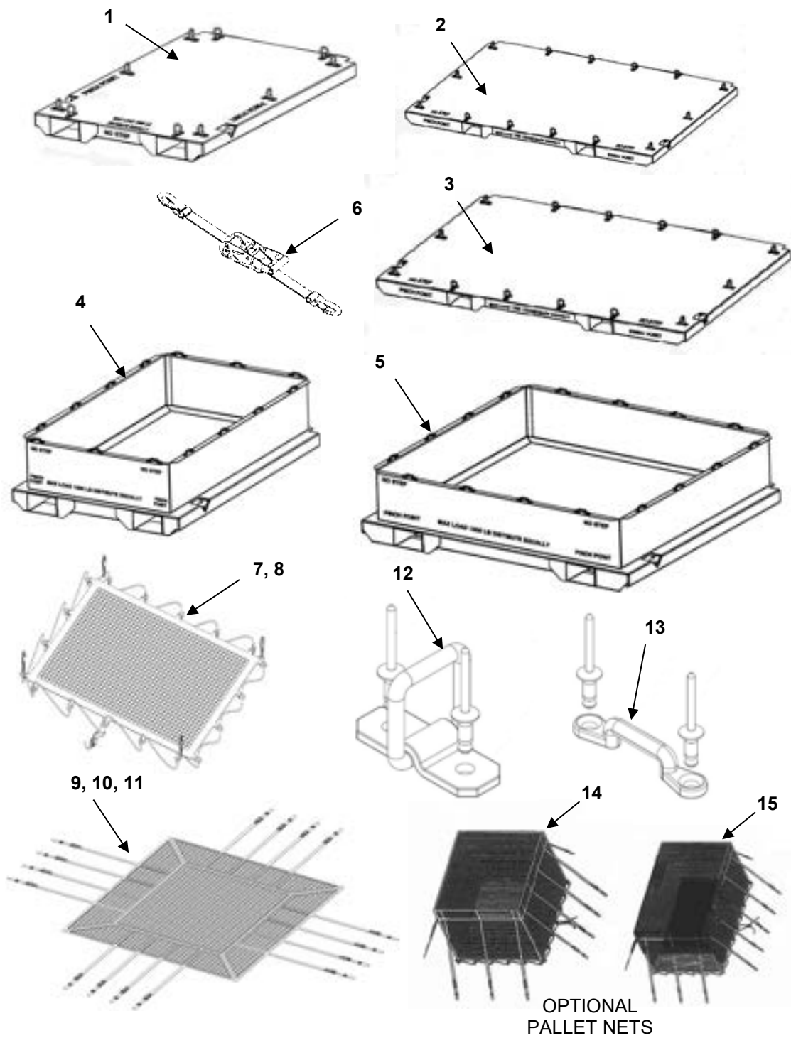
FIGURE 15 PALLETS
