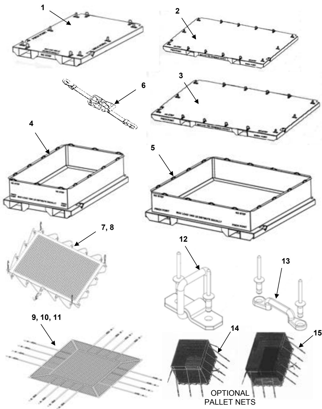
FIGURE 27 PALLETS
