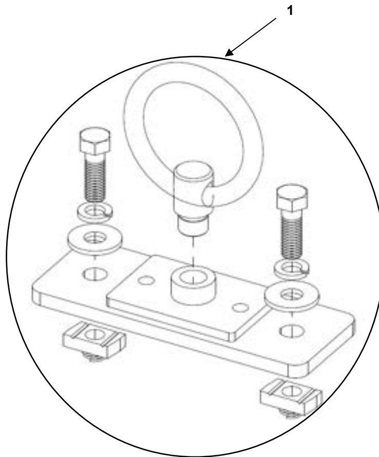
FIGURE 52 TIE DOWN RING ASSEMBLY
