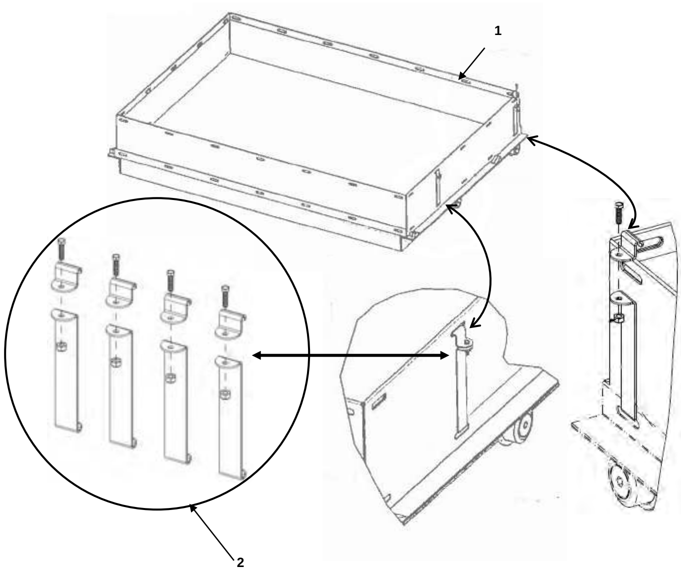
FIGURE 46 BULK 8" BIN ADAPTER KIT
