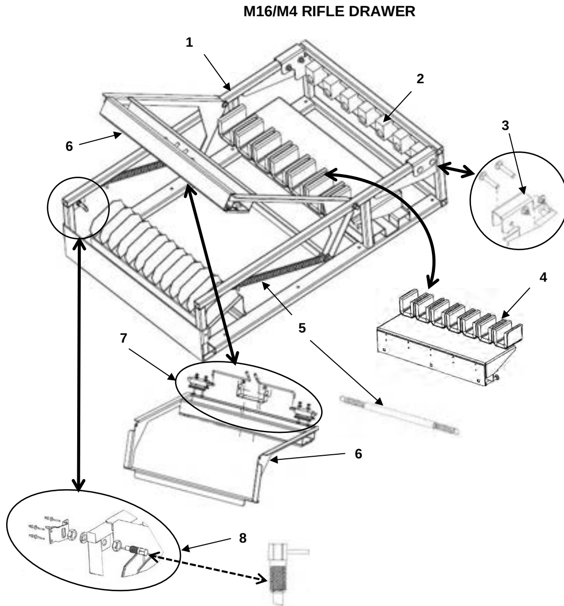
FIGURE 35 M16/M4 RIFLE DRAWER
