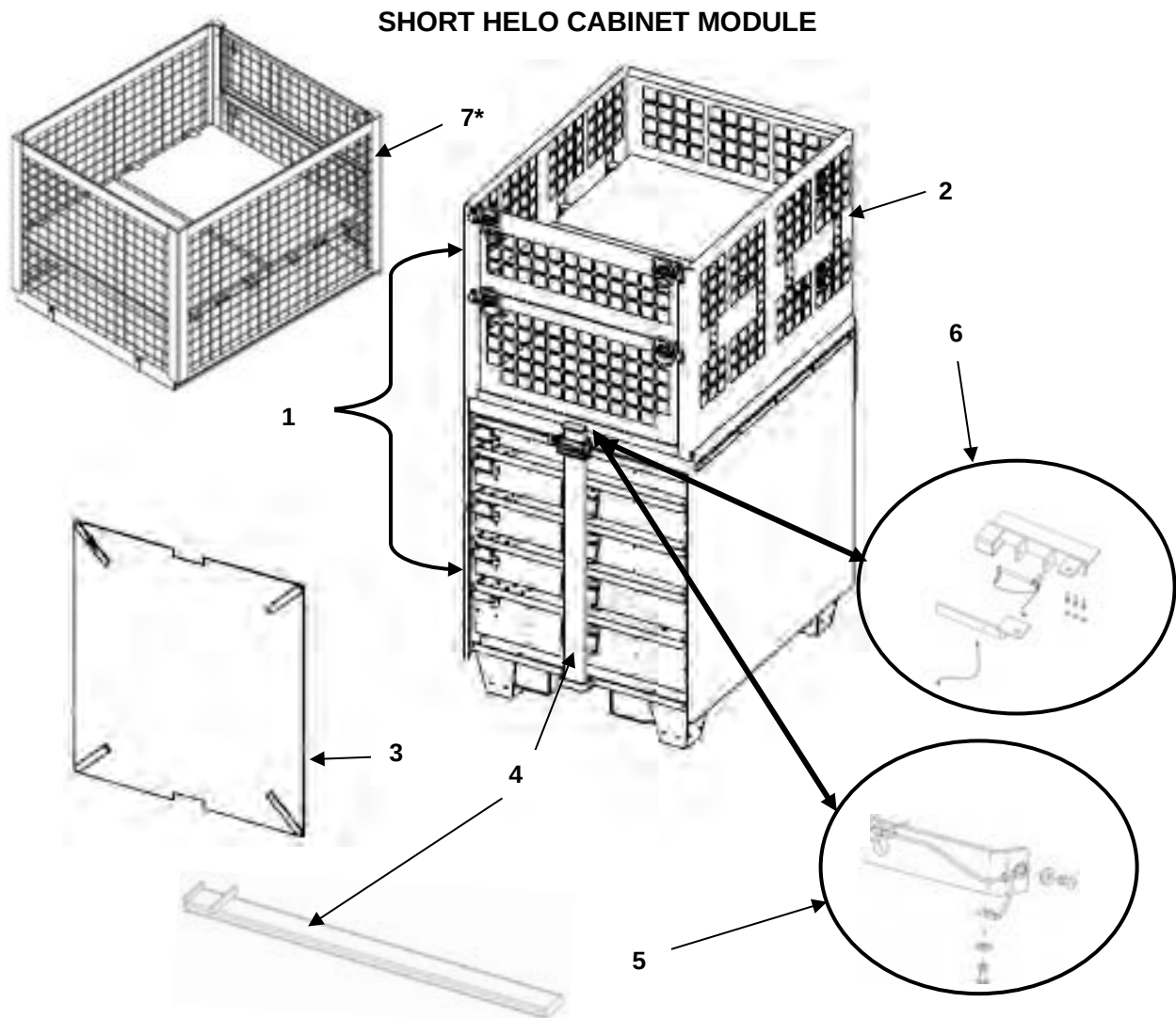
FIGURE 25 SHORT HELO CABINET MODULE WITH CAGE NOTE
