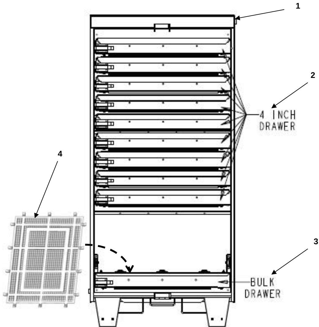
FIGURE 20 STANDARD MODULE #17 CLASS 6 COVER AND RETAINING BAR REMOVED FOR CLARITY
