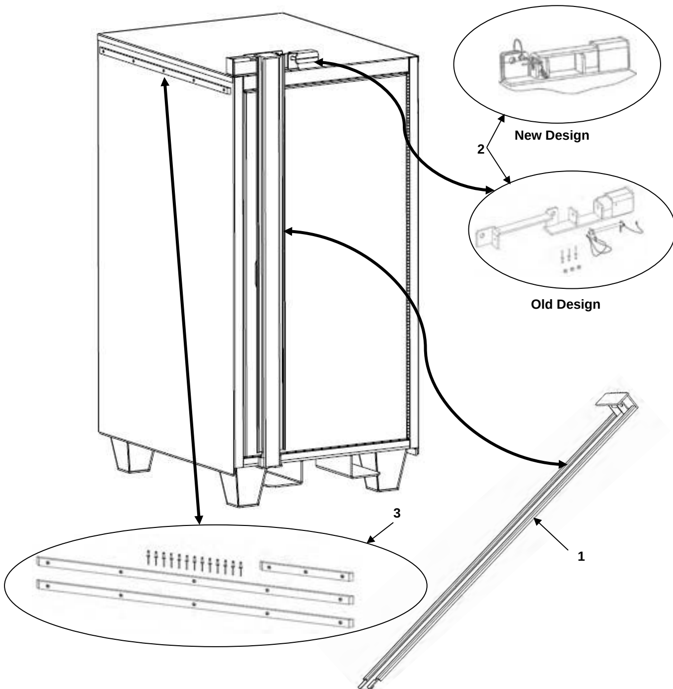
FIGURE 30 WEAPONS VAULT MODULE
