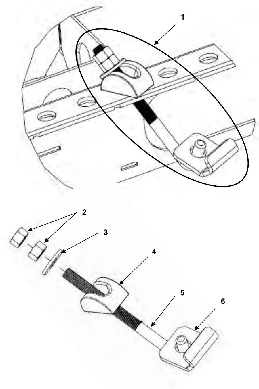
FIGURE 50 HOOK BOLT AND PLATE KIT
